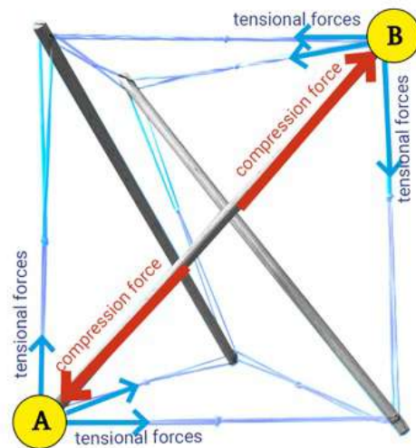
Fig. 16. Set of forces acting on one rod (between point A and B). Tension element (blue arrows) pulling inwards while compression force (red arrows) push outwards. With the right ratio length between the rods and tendons the model becomes balanced.
